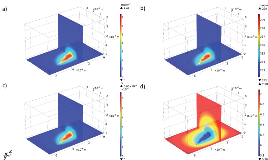
Fig. 9 3D multi-slice plots produced in COMSOL showing the final (at a time of 0.5 s): (a) concentration of Fe 2+ ions, (b) concentration of Cl - ions, (c) electrolyte potential, and (d) pH.
