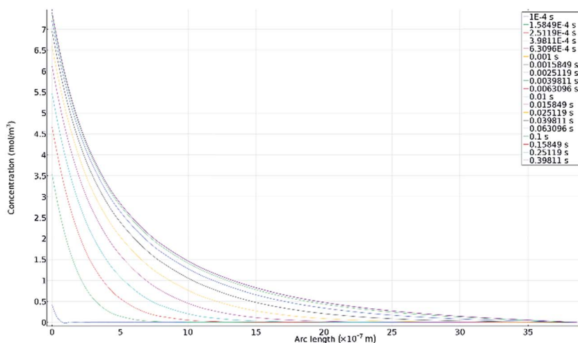
Fig. 10 A line plot produced in COMSOL showing the concentration of Fe 2+ ions along a line normal to the metal surface, starting from the centre of the pit and extending out to the bulk solution, for different time steps.
