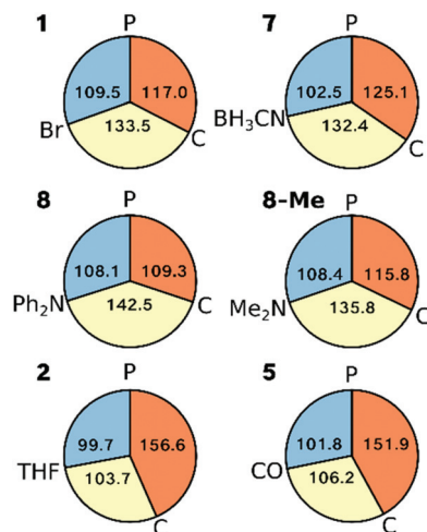
Fig. 9 Pie diagrams representing the angles around the Ni ion in the crystal structures for 1 , 2 , 5 , 7 , 8 and the geometry optimised structure of 8-Me ; orange: ∠P–Ni–C, yellow: ∠C–Ni–L, blue: ∠L–Ni–P, where L stands for the respective ligand.
