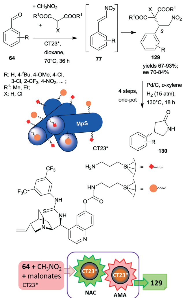
Scheme 36 One-pot cascade nitroaldol condensation (NAC) and AMA catalysed by the multifunctional chiral catalyst and transformation of the products in a consecutive one-pot four step reaction over \text{Pd/C} ; Mps: mesoporous silica. 180,181
