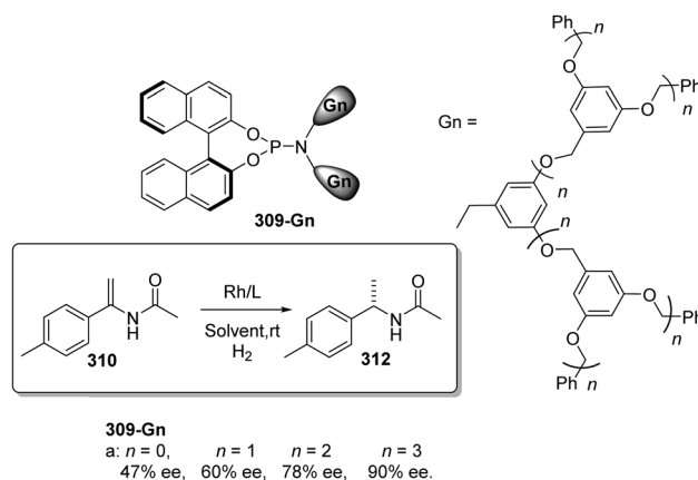
Fig. 76 Dendritic chiral monodentate phosphoramidite ligands developed for enantioselective Rh-catalyzed hydrogenations.
