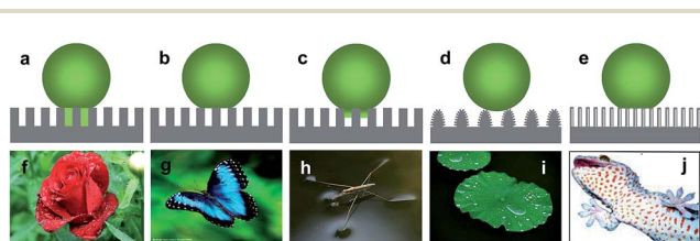
Fig. 2 Five typical cases for anti-wetting surfaces (a: Wenzel state; b: Cassie state; c: Wenzel–Cassie state; d: “lotus” state; e: “gecko” state) and several common phenomena for anti-wetting in nature (f: petal; g: butterfly; h: strider; i: lotus leaf; j: gecko).
