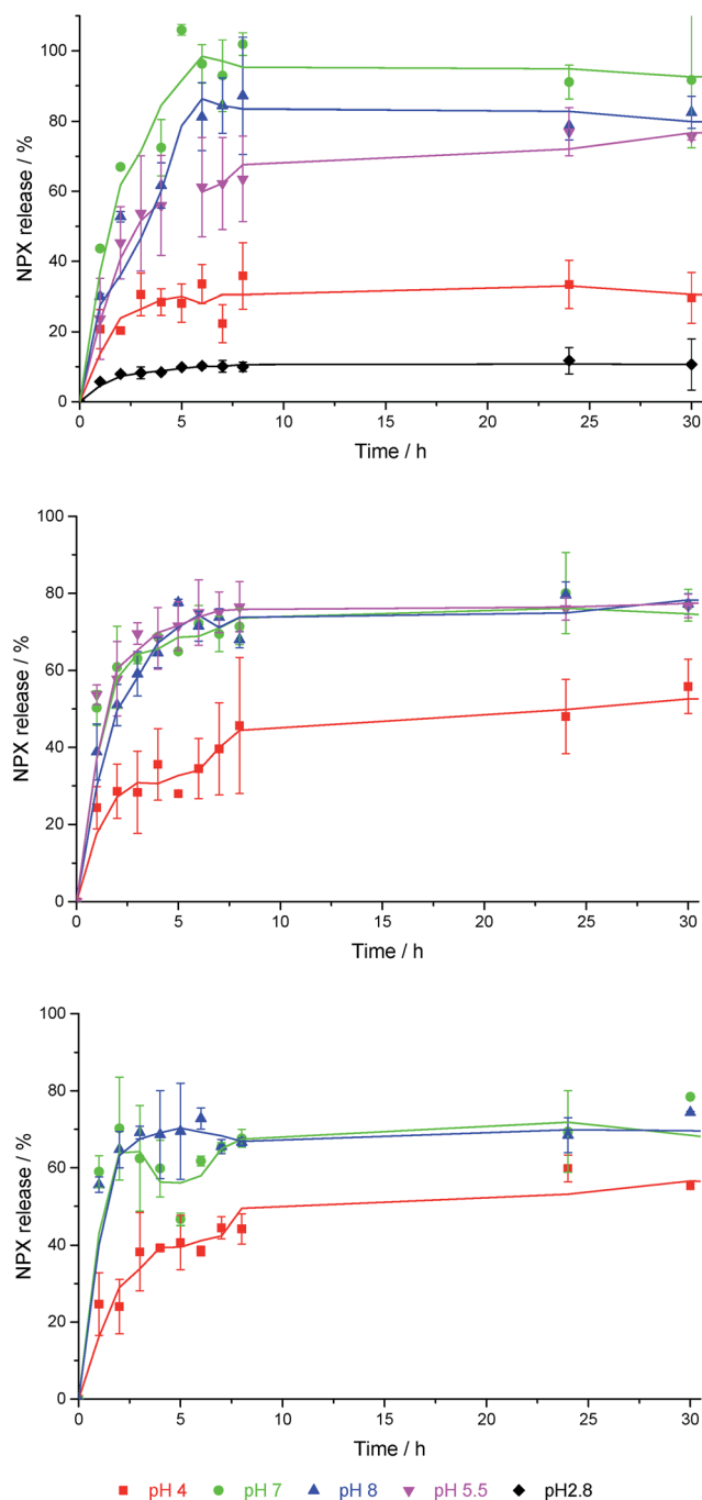
Fig. 5 NPX release profiles for (top) 6 mM DBS-CONHNNH 2 , (centre) 5% hybrid gel, and (bottom) 10% hybrid gel, into buffer solutions with different pH values in each case.
