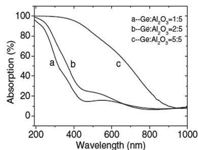
Fig. 5 Optical absorption spectra of Ge nanocrystals embedded in Al 2 O 3 films on quartz substrates (synthesized at room temperature; thickness: 200 nm). 72
