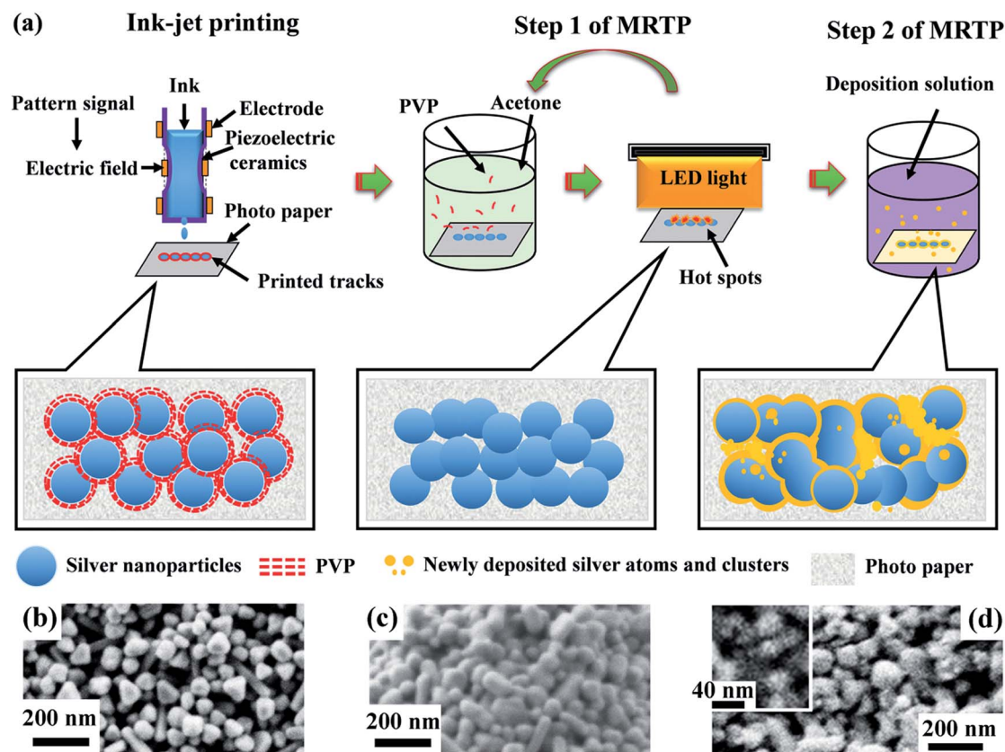
Fig. 3 (a) Schematic representation of MRTTP. SEM images show the morphologies of the silver tracks at different steps. (b) Before sintering, (c) treated by the Step 1 of MRTP and (d) treated by Step 2 of MRTP. The inset in (d) shows the high resolution image of small nanoparticles newly deposited on to the silver track.
