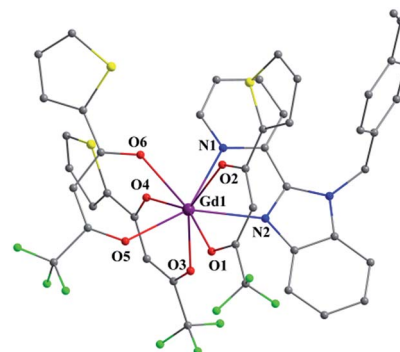
Fig. 1 Perspective drawing of complex monomer [\text{Gd}(\text{TTA})_3(4\text{-VP-PBI})] ( 4 ); H atoms have been omitted for clarity.
