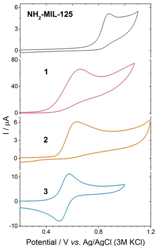
Fig. 4 Cyclic voltammetry at 50\text{ mV s}^{-1} of \text{NH}_2\text{-MIL-125(Ti)} , 1 , 2 (phosphate buffer, pH 7) and 3 ( 0.1\text{ M LiClO}_4 ) in water as it is the only medium that allowed for electrochemical measurements of the MOF.
