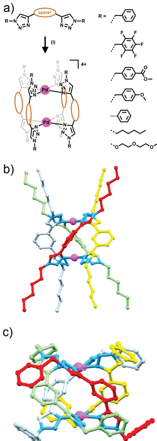
Fig. 7 (a) Generic scheme showing the formation of [Pd_2L_4]^{4+} helicates from bis-monodentate 1,2,3-triazole ligands, Linker = 1,3-phenyl, 1,4-phenyl or propyl, (i) [Pd(CH_3CN)_2](BF_4)_2 , CH_3CN , RT or 70\text{ }^\circ\text{C} ; (b) MMFF model of the hexyl-substituted [Pd_2L_4]^{4+} helicate which exhibited biological activity; (c) X-ray structure of the benzyl-substituted [Pd_2L_4](BF_4)_4 helicate. Counterions, solvent molecules and hydrogen atoms have been omitted for clarity.
