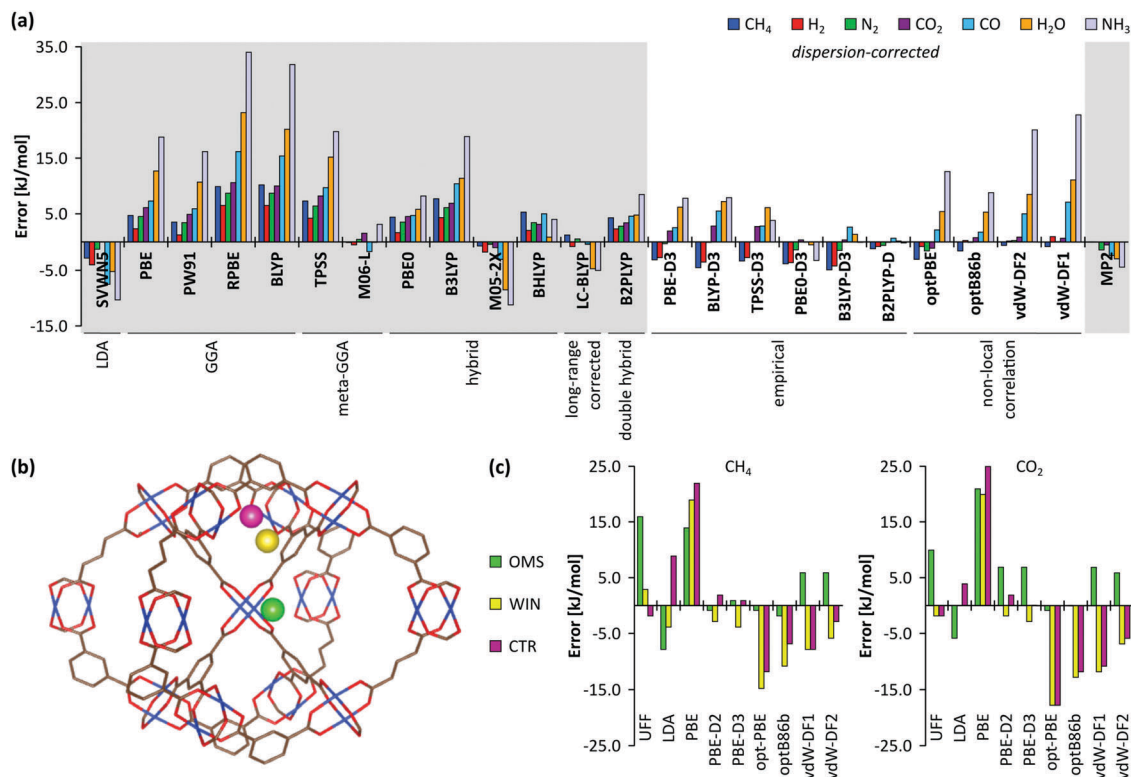
Fig. 14 (a) Errors in the interaction energies of adsorbate-Cu(HCOO) 2 calculated with respect to CCSD(T)/CBS level of theory; (b) the CuBTC supercage with indication of an open metal site (OMS, green), a tetrahedral cage-window site (WIN, yellow) and a tetrahedral cage-centre site (CTR, magenta) as the three main adsorption sites; (c) errors in the interaction energies calculated for CH 4 and CO 2 at the three main adsorption sites with respect to the DFT/CC reference level of theory. Figure adapted from ref. 253 with permission from the American Chemical Society, copyright 2015.
