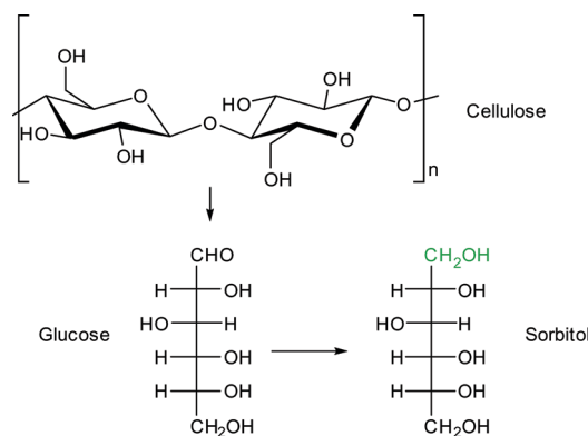
Scheme 2 Cellulose and cellobiose into sorbitol.
