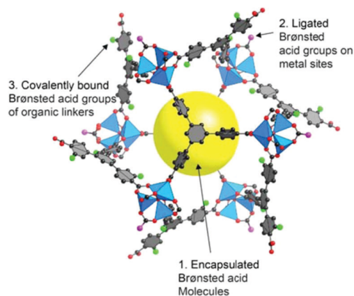
Fig. 11 Various Brønsted-acid sites in MOFs. Reprinted from ref. 107. Copyright 2015 with permission from the American Chemical Society.
