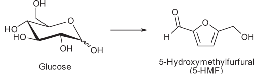
Scheme 4 Conversion of glucose to 5-HMF.
