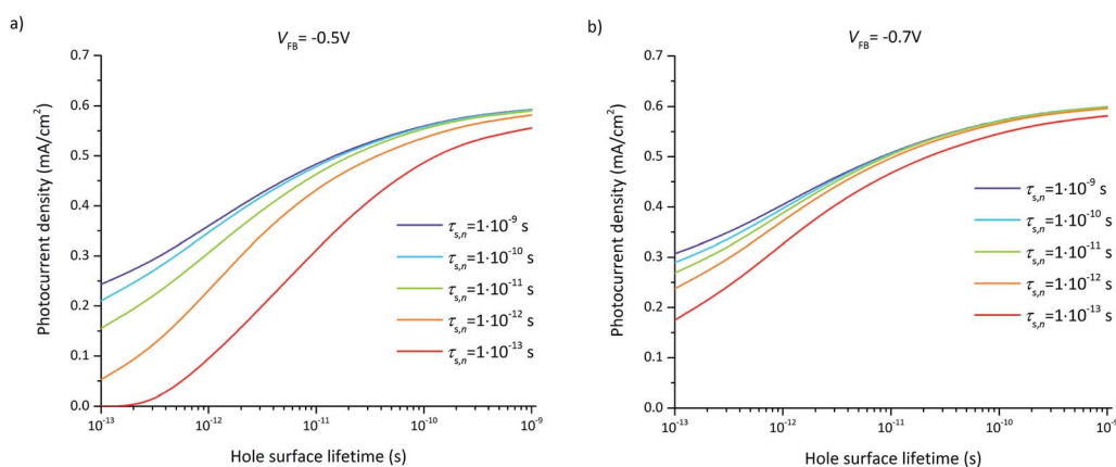
Fig. 11 Photocurrent density at 0.3 V vs. RHE as a function of the hole surface lifetime for various electron lifetimes ( \tau_{s,n} = 10^{-9} , 10^{-10} , 10^{-11} , 10^{-12} , 10^{-13} s) and two flatband potentials: (a) V_{FB} = -0.5 V vs. RHE, and (b) V_{FB} = -0.7 V vs. RHE.
