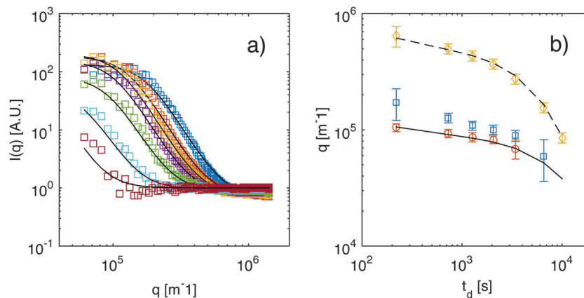
Fig. 5 (a) Scattering intensity I_r(q) obtained for a diffusing colloidal suspension at various times t_d from the beginning of diffusion: t_d = 180, 690, 1230, 2010, 3390, 6540, and 10\,000 s (from top to bottom). Continuous lines are best fits to eqn (9). Data for I_s(q) are shown in ESI† (b) Roll-off wave-vector q_{co} as a function of the time t_d elapsed from the beginning of diffusion, as obtained from the static (blue squares) and from the dynamic (orange circles) analysis of the NEF. The continuous line is a theoretical prediction from eqn (11), evaluated for z corresponding to the sample mid-plane. Yellow diamonds represent the crossover wave-vector q_{co} . The dashed line is the theoretical prediction from eqn (12), again calculated for z corresponding to the sample mid-plane. In addition, the osmotic compressibility \bar{\chi} is assumed to remain constant during diffusion.
