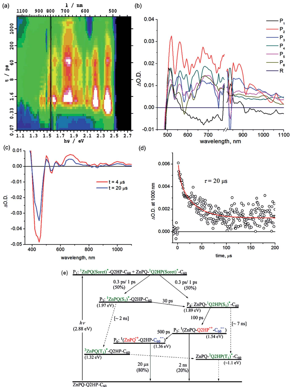
Fig. 3 Transient absorption spectra of \text{ZnPQ-Q2HP-C}_{60} following excitation at 430 nm in PhCN at 298 K: (a) \Delta A(\nu, t) at frequency \nu following femtosecond laser pulse irradiation at prior time t ; (b) component spectra P_i(\nu) (shown as a function of wavelength); (c) 4 and 20 \mu\text{s} after nanosecond laser pulse; (d) the time-decay profile of the optical density at 1000 nm; and (e) the reaction scheme used with fitted process lifetimes \tau . Dotted lines indicate expected but unobserved processes.
