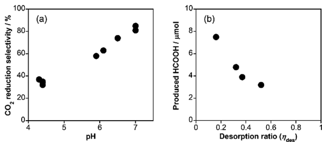
Fig. 4 (a) Selectivity of CO 2 reduction ( \text{sel}_{\text{CO}_2} ) vs. pH of the reaction solution in the photocatalytic reactions. (b) Produced amount of HCOOH vs. desorption ratio of RuRu ( \eta_{\text{des}} ) by the photocatalytic reactions with various concentration of NaH 2 PO 4 (pH = 4.4).
