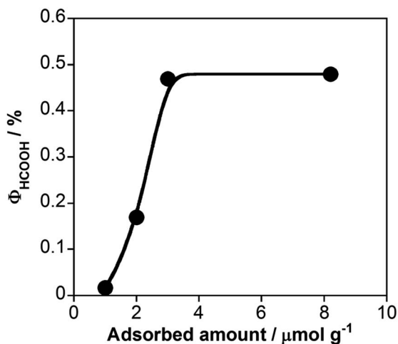
Fig. 5 Relationship between \Phi_{\text{HCOOH}} and loading amount of RuRu in the photocatalytic reaction using RuRu/Ag/TaON (30 mg) and EDTA·2Na (10 mM) in aqueous solution (10 mL) with 400 nm monochromatic light irradiation under a CO 2 atmosphere.
