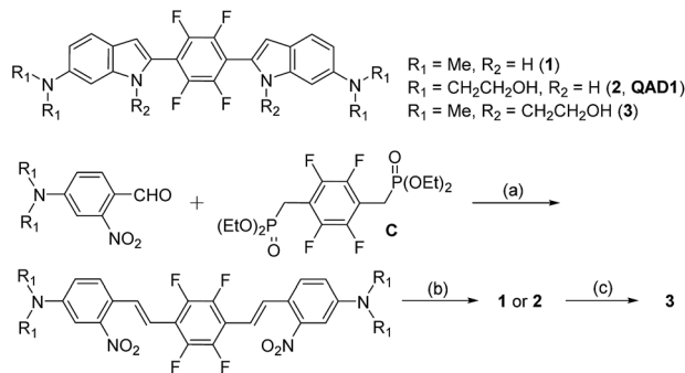
Scheme 1 Chemical structures of 1–3 and their synthetic route: Reagents and conditions: (a) \text{KO}^t\text{Bu} , THF, 0-20^\circ\text{C} ; (b) \text{P}(\text{OEt})_3 , 125^\circ\text{C} ; (c) i: compound 1 , 2-bromoethylacetate, NaH, 18-Crown-6, THF, 80^\circ\text{C} ; ii: NaOMe, \text{CH}_3\text{OH} , 0-20^\circ\text{C} .
