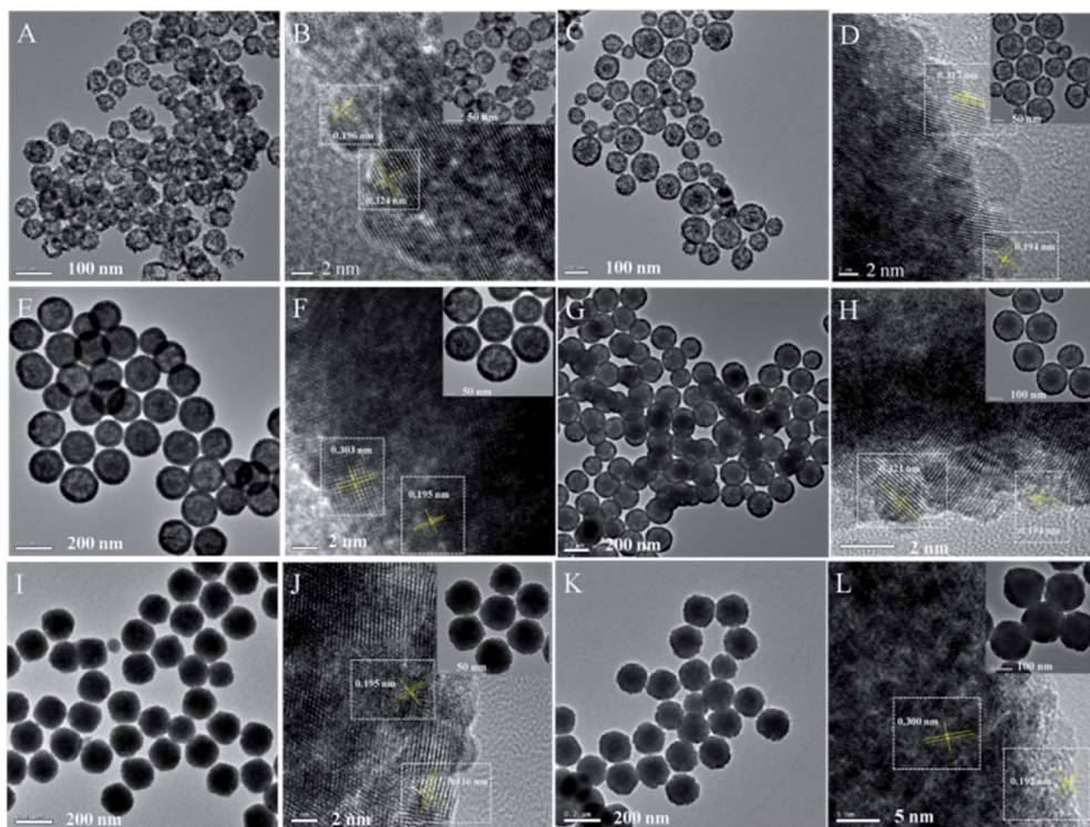
Fig. 3 TEM images of (A) and (B) Cu–CeO 2 –Pt; (C) and (D) Cu 0.66 Co 0.34 –CeO 2 –Pt; (E) and (F) Cu 0.50 Co 0.50 –CeO 2 –Pt; (G) and (H) Cu 0.34 Co 0.66 –CeO 2 –Pt; (I) and (J) Co–CeO 2 –Pt; (K) and (L) CeO 2 –Pt.
