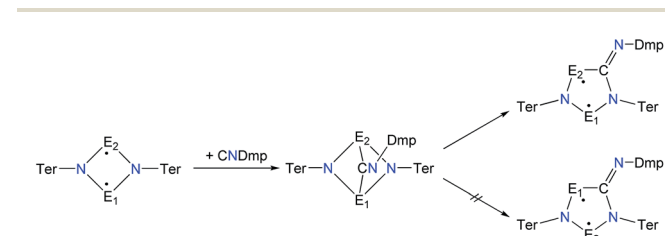
Scheme 7 Proposed reaction mechanism for isonitrile activation with 1E 1 E 2 ( E^1 is lighter than E^2 ).
