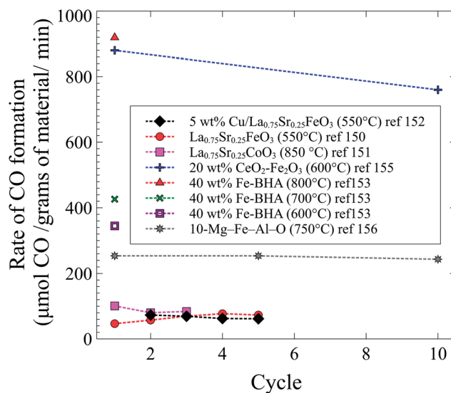
Fig. 5 \text{CO} formation as a function of cycle in the intensified rWGS-CL process from ref. 150–153, 155 and 156.
