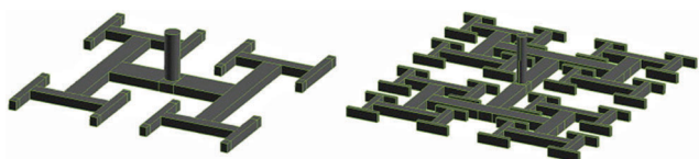
Fig. 8 Fractal design with 16 and 64 outlets used for modeling studies. 98 Reprinted from ref. 98 with permission from Elsevier.
