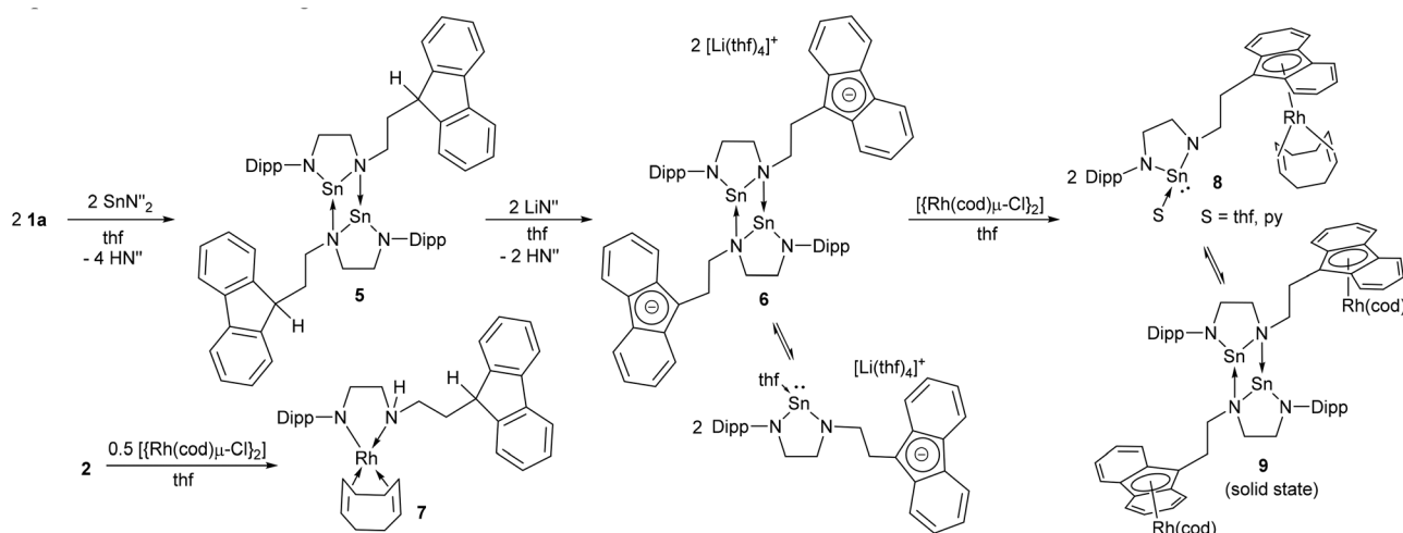
Scheme 3 Synthesis of N-heterocyclic stannylenes and Rh complexes ( \text{N}'' = \text{N}(\text{SiMe}_3)_2 , \text{cod} = 1,5\text{-cyclooctadiene} ).
