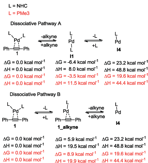
force for the dissociation of L is greater going through pathway A over pathway B. Furthermore, the breaking of the second Pd–L bond to form the reactive mono-ligand Pd(0)–L ( I4 ) is easier for L = PMe 3 , than for L = NHC systems. Indeed, the
