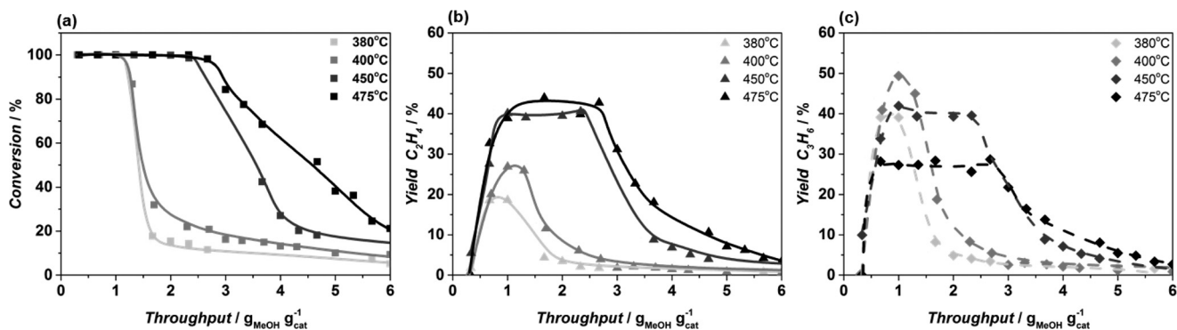
Fig. 5 Methanol conversion (a), yield of ethylene (b) and propylene at 380 °C (□, △, ◇), 400 °C (■, ▲, ◆), 450 °C (▣, ▤, ▥) and 475 °C (■, ▲, ◆) obtained in MTO reaction over Sigma1-315-M zeolite with SiO 2 /Al 2 O 3 = 315 and crystal size of 2.5 μm at standard operation conditions.
