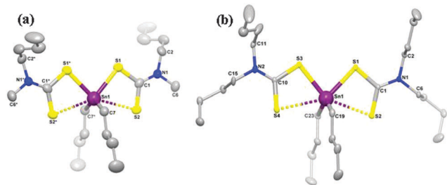
Fig. 10 Molecular structures of (a) [\text{Sn}(\text{C}_4\text{H}_9)_2(\text{S}_2\text{CNMe}^t\text{Bu})_2] and (b) [\text{Sn}(\text{C}_4\text{H}_9)_2(\text{S}_2\text{CN}^t\text{Bu})_2] with 50% ellipsoidal probability level. All the H atoms on carbon frames are removed for clarity. Reproduced with permission from ref. 97. Copyright 2014 American Chemical Society.
