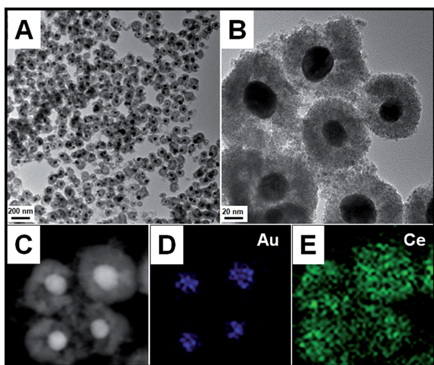
Fig. 2 TEM (A and B), and HAADF-STEM images (C to E) of Au@CeO 2 .
