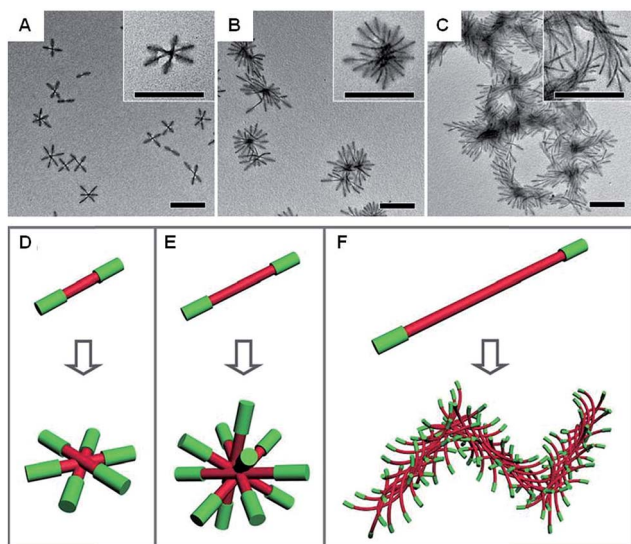
Fig. 10 Schematic representations and corresponding TEM images of the hierarchical self-assembly of amphiphilic B-A-B triblock comicelles. \text{M(PFS-}b\text{-P2VP)-}b\text{-M(PFS-}b\text{-PDMS)-}b\text{-M(PFS-}b\text{-P2VP)} (P2VP = poly(2-vinylpyridine)) with B block lengths of 90 nm and different A block lengths of 110 (A), 260 (B) and 505 nm (C) after dialysis from hexane/isopropanol against pure isopropanol. (D–F) Schematics of the supermicelles formed. For simplicity, the A and B blocks are represented as red and green cylinders, respectively. Scale bars correspond to 500 nm. Reproduced with permission from ref. 106.
