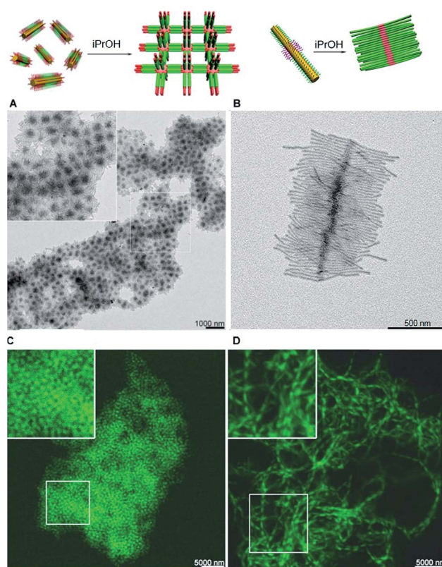
Fig. 11 Supermicelles and superlattices by stacking of A-B-A and B-A-B triblock comicelles (A = \text{M(PFS-}b\text{-P2VP)} and B = \text{M(PFS-}b\text{-PDMS)} ). (A) TEM images of a 3D superlattice formed by \text{A}_{105\text{ nm}}\text{-B}_{160\text{ nm}}\text{-A}_{105\text{ nm}} triblock comicelles. (B) TEM images of a cylindrical brush-like supermicelle formed by \text{B}_{340\text{ nm}}\text{-A}_{35\text{ nm}}\text{-B}_{340\text{ nm}} triblock comicelles in iPrOH. (C) Confocal fluorescence microscopy images of a 3D superlattice formed by \text{A/F}_{300\text{ nm}}\text{-B}_{570\text{ nm}}\text{-A/F}_{300\text{ nm}} triblock comicelles in iPrOH (F = hydrophobic fluorescent block copolymer). (D) Confocal fluorescence microscopy images of a 1D superlattice formed by \text{A/F}_{745\text{ nm}}\text{-B}_{570\text{ nm}}\text{-A/F}_{745\text{ nm}} triblock comicelles in iPrOH. Reproduced with permission from ref. 107.
