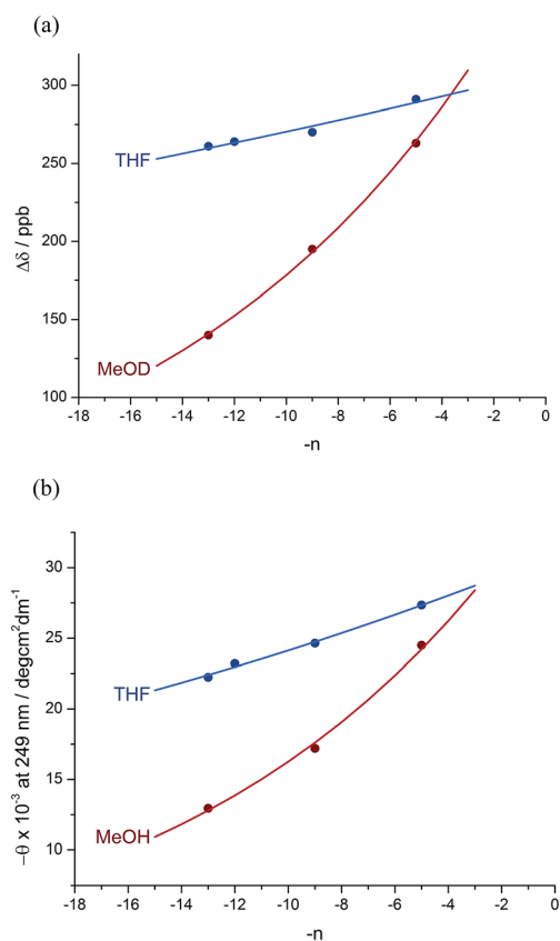
Fig. 10 Effect of chain length n on characteristic features of the products 8a–d . (a) Exponential decay of anisochronicity in the azepine \text{CH}_2 groups with chain length ( \bullet in THF at 23 °C; \text{—} f = 0.013 ; \bullet in methanol at 23 °C; \text{—} f = 0.077 ); (b) exponential decay of molar ellipticity at 249 nm ( \bullet in THF at 23 °C; \text{—} f = 0.025 ; \bullet in methanol at 23 °C; \text{—} f = 0.076 ).
