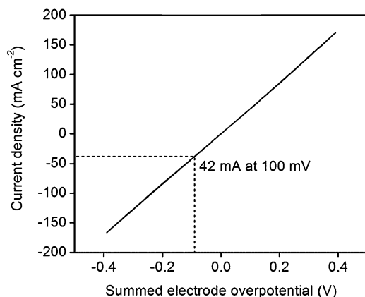
Fig. 8 IR-corrected polarization curve of a 46 wt% Pt-CNT- \text{CsH}_2\text{PO}_4 composite electrode at 1 \text{ mV s}^{-1} , showing high current density at low overpotentials for both proton reduction and hydrogen oxidation.
