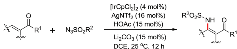
Scheme 306 The iridium-catalyzed intermolecular C–H amidation of ketone derivatives.
