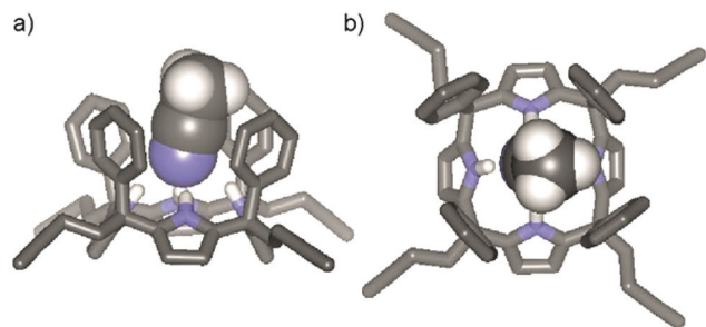
Fig. 2 (a) Side view and (b) top view of the X-ray structure of the aryl extended calix[4]pyrrole \text{CH}_3\text{CN} at \alpha,\alpha,\alpha,\alpha-3 . For clarity, non-polar hydrogen atoms have been omitted. The included acetonitrile molecule is shown in CPK representation.
