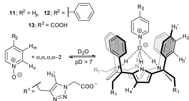
Fig. 3 Equilibrium involved in the formation of the inclusion complexes PNO at \alpha,\alpha,\alpha,\alpha-2 and the proposed structure for the binding geometry.
