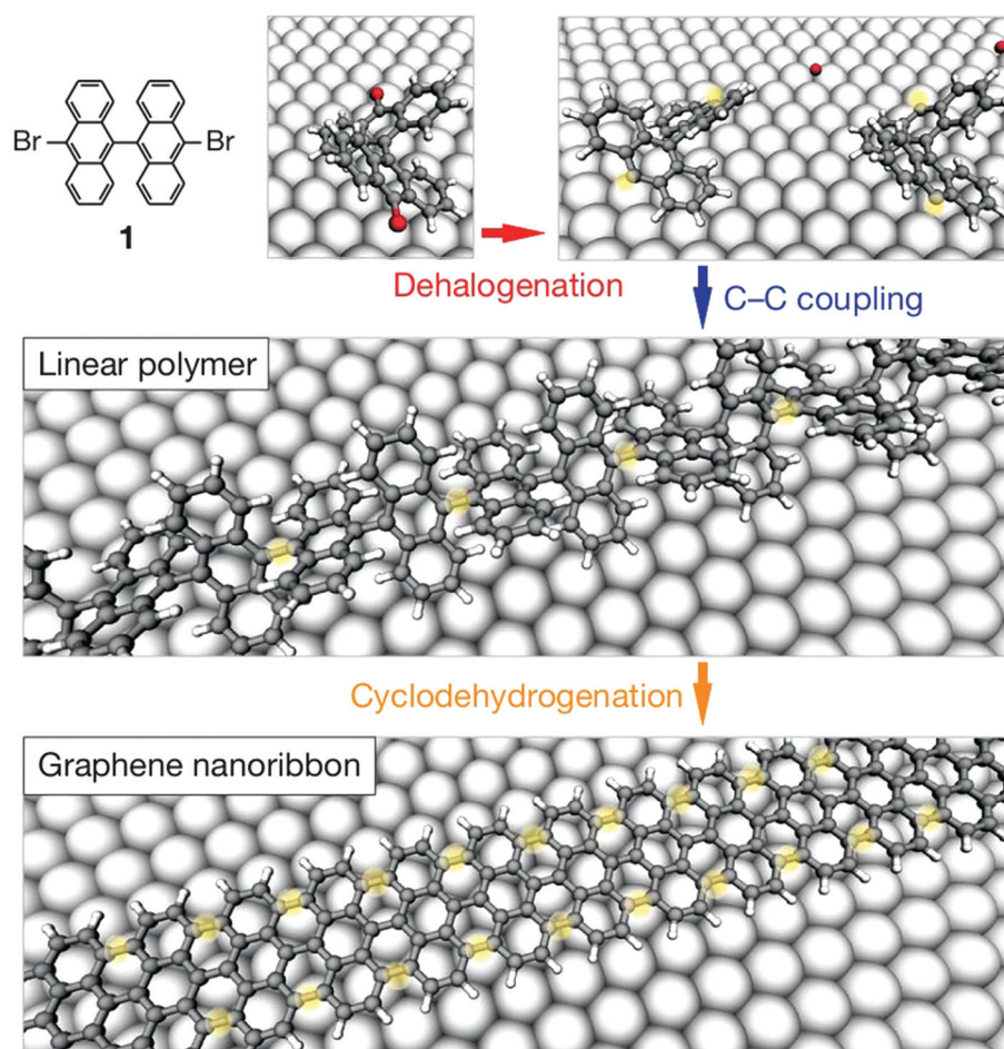
Fig. 48 Bottom-up fabrication of synthetic graphene and GNRs starting from 10,109-dibromo-9,99-bianthryl monomers ( 1 ). Top, dehalogenation during adsorption of the precursor monomers. Middle, formation of linear polymers by covalent interlinking of dehalogenated intermediates. Bottom, formation of fully aromatic GNRs by cyclodehydrogenation. 320
