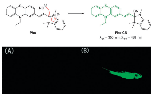
Fig. 31 Top: reaction of \text{CN}^- with indolium Phc . Bottom: images of adult zebrafish under 390 nm light: (A) fish incubated with Phc ; (B) fish incubated with Phc and \text{CN}^- . Image reproduced with permission. 177
