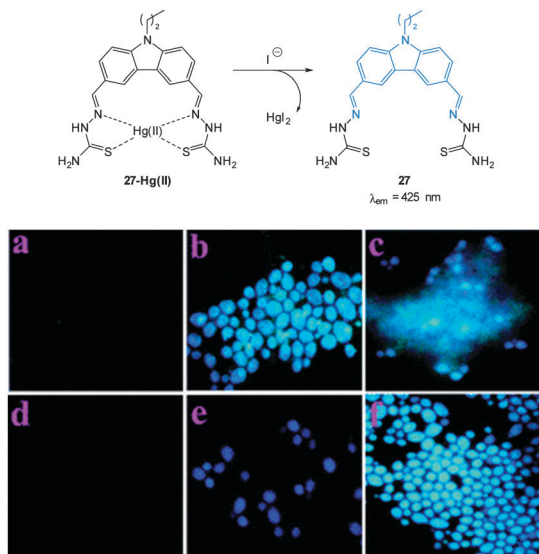
Fig. 24 Top: structure and reaction of iodide probe 27-Hg(II) ; bottom: fluorescence images of Candida albicans (a) cells only, (b) cells with 27 , (c) cells with 27 after addition of \text{Hg(II)} (5 \mu\text{M} ), (d) cells with 27 and \text{Hg(II)} (25 \mu\text{M} ), (e) cells with the preformed 27-Hg(II) complex and KI, (f) same as (e) after 10 min. Image used with permission. 162
