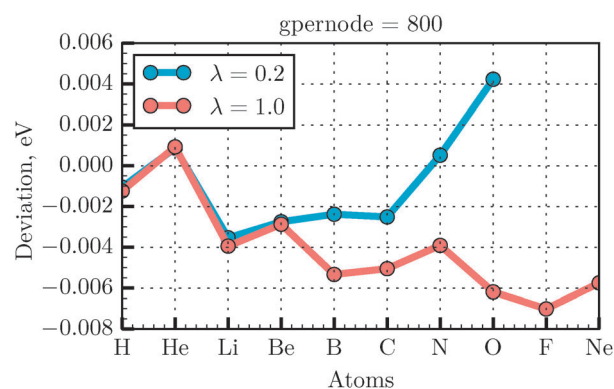
Fig. 4 Energy deviation with respect to the reference value 32 calculated for the first and second row elements for gpnnode = 800 , \lambda = 0.2, 1.0 , and rcut = 1.2 Bohr.
