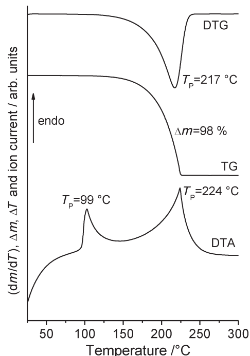
Fig. 11 DTA, TG and DTG curve for form 1t at 4 °C min -1 in a nitrogen atmosphere.
