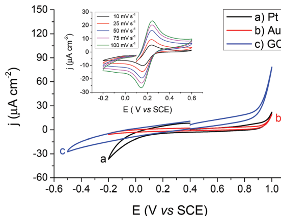
Fig. 4 Blank CVs of 10 mM BTTPATPBCl electrolyte in 5-nonanone solvent measured on 2.07 mm, 2.11 mm and 3.06 mm diameter Pt, Au and GC disc electrodes, respectively. Voltammetric responses of 200 \mu M TCNQ on the Au disc electrode is shown in the inset.
