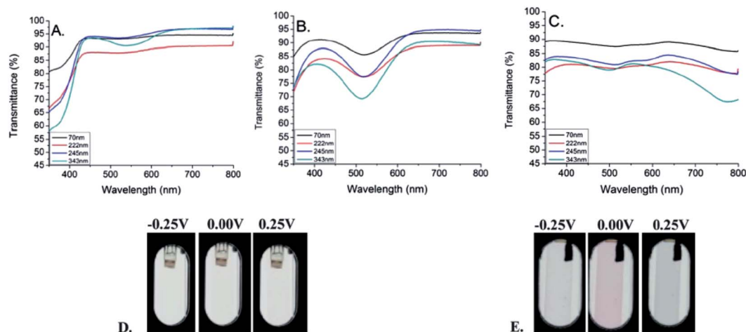
Fig. 9 UV/Vis-NIR transmittance spectra for the neutral (A), intermediate (B), and oxidized (C) states of PProDOP- N -C 18 H 37 of increasing thickness, spray-cast onto ITO glass. Images show the films of 70 nm (D) and 343 nm (E) thickness at the voltages indicated. 79
