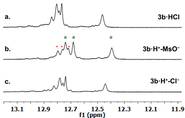
Fig. 4 ^1\text{H} NMR spectra in \text{CDCl}_3 for the pyrrolic NH region of: (a) 3\text{b}\cdot\text{HCl} ; (b) after addition of 6 eq. of MsOH to sample a, two sets of NH signals were observed for each \alpha (·) and \beta (*) conformer; (c) after addition of 1 eq. of tetrabutylammonium chloride (TBACl) to sample b.
