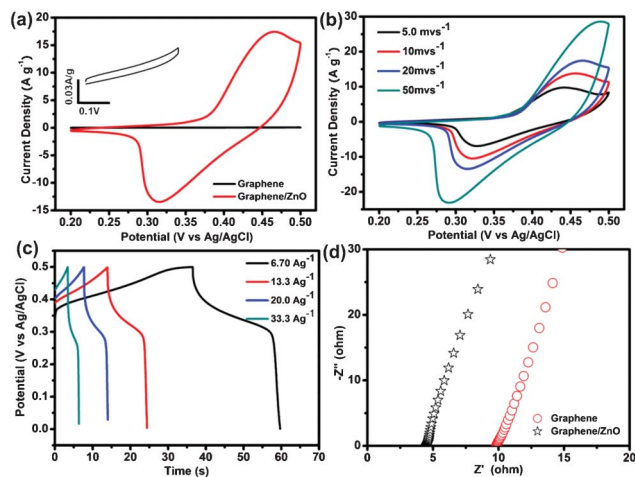
Fig. 5 (a) CV curves of free-standing graphene and graphene/ZnO hybrid electrodes at a scan rate of 20 \text{ mV s}^{-1} in 2.0 M KOH electrolyte. The inset shows the enlarged CV curve of a graphene foam electrode. (b) CV curves of the graphene/ZnO hybrid electrode at different scan rates of 5 \text{ mV s}^{-1} , 10 \text{ mV s}^{-1} , 20 \text{ mV s}^{-1} , and 50 \text{ mV s}^{-1} . (c) Galvanostatic charge-discharge curves of the graphene/ZnO hybrid electrode at different current densities. (d) Nyquist plots of graphene foam and graphene/ZnO hybrid electrodes.
