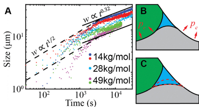
Fig. 8 Compare with experimentally measured growth dynamics of osmocapillary phase separation (A) experimental data agrees with the w \propto t^{0.32} (solid black lines) scaling at long time scales when linear deformation assumption is valid. Relaxation is faster than both t^{0.32} and the conventional t^{1/2} (dashed black lines) at short time scales when nonlinear effect is significant. Same colors correspond to the same data set in Fig. 7. (B) With significant nonlinear deformation, capillary pressure on the surface promotes the solvent migration towards the surface, thus accelerating the relaxation. (C) With significant nonlinear deformation, the flux into the osmocapillary phase separation mainly fills the volume occupied by the deformed solid (encircled by red dashed line) rather than increasing the curvature of the solvent surface, thus not reducing the capillary pressure in the phase separation, leading to faster relaxation.
