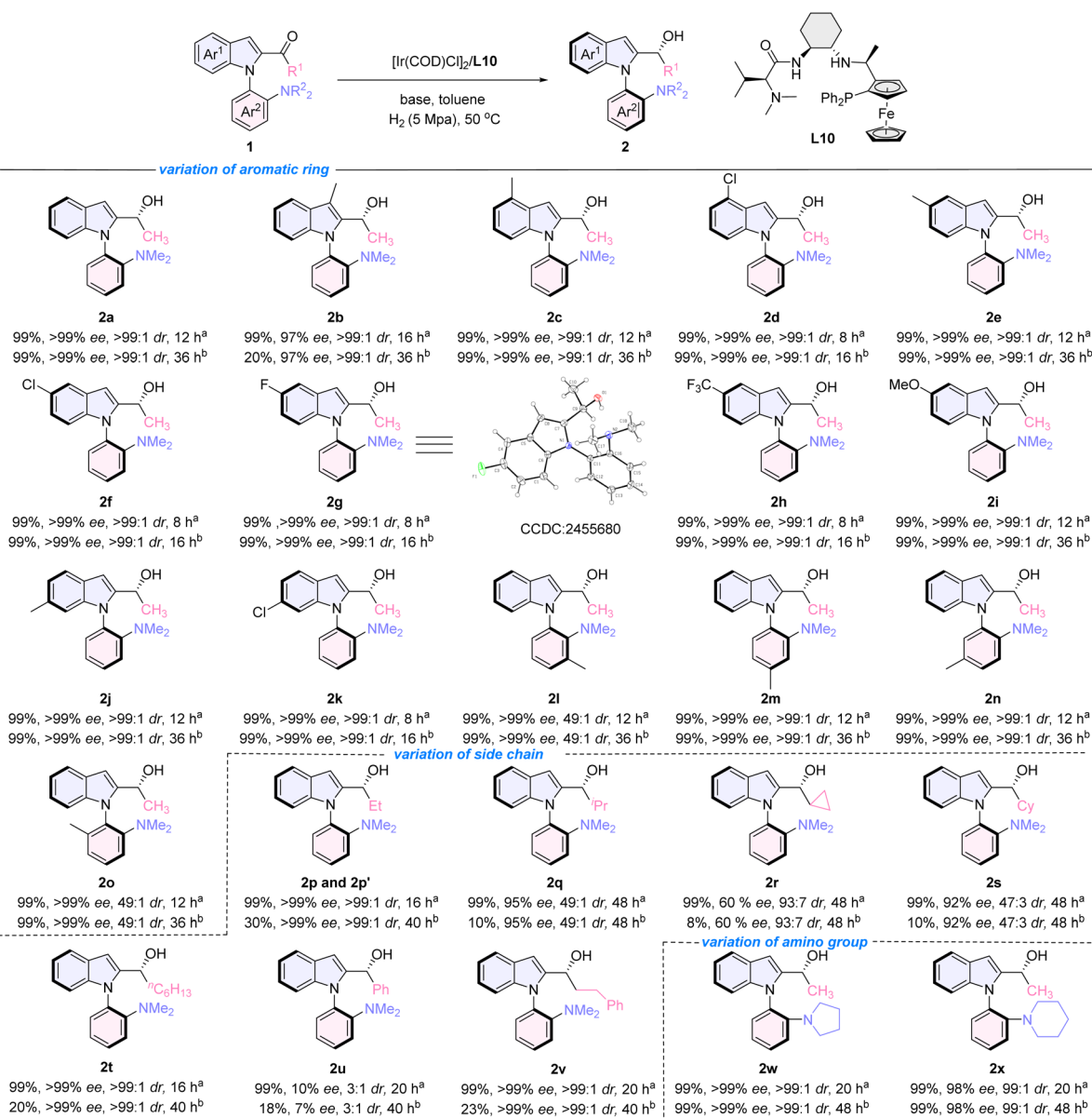
Scheme 2 Substrate scope of N -aryl indole ketones. a Reaction conditions: 1 (0.25 mmol), [\text{Ir}(\text{COD})\text{Cl}]_2 (0.05 mol%), L10 (0.11 mol%), \text{Cs}_2\text{CO}_3 (10 mol%), toluene (1 mL), 50 °C and \text{H}_2 (5 MPa). Isolated yields were obtained by flash chromatography and the ee and dr values were determined by HPLC analysis. b \text{CH}_3\text{CO}_2\text{Li} was used as the base instead of \text{Cs}_2\text{CO}_3 .
