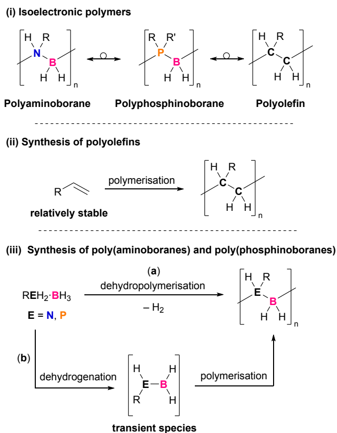
Scheme 1: Overview of the structure (i) and synthesis of poly(olefins) (ii), and poly(aminoboranes) and poly(phosphinoboranes) (iii). Pathway (a) described the direct dehydropolymerisation typical of the transition-metal catalysed dehydropolymerisation of phosphine-borane adducts and pathway (b) describes two-step dehydropolymerisation where initially dehydrogenation of the precursor occurs, followed by polymerization of reactive species formed in situ , typical of the transition-metal catalysed dehydropolymerisation of amine-borane adducts.
