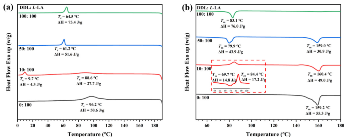
Fig. 4 DSC thermograms of (a) the cooling run with a cooling rate of 10\text{ °C min}^{-1} and (b) the second heating run with a heating rate of 10\text{ °C min}^{-1} for different [\text{DDL}]_0/[\text{L-LA}]_0 ratios. [\text{DDL}]_0/[\text{L-LA}]_0 = 100:100 (Table 2, run 5); [\text{DDL}]_0/[\text{L-LA}]_0 = 50:100 (Table 2, run 4); [\text{DDL}]_0/[\text{L-LA}]_0 = 10:100 (Table 2, run 3); neat PLLA (Table 2, run 1).
