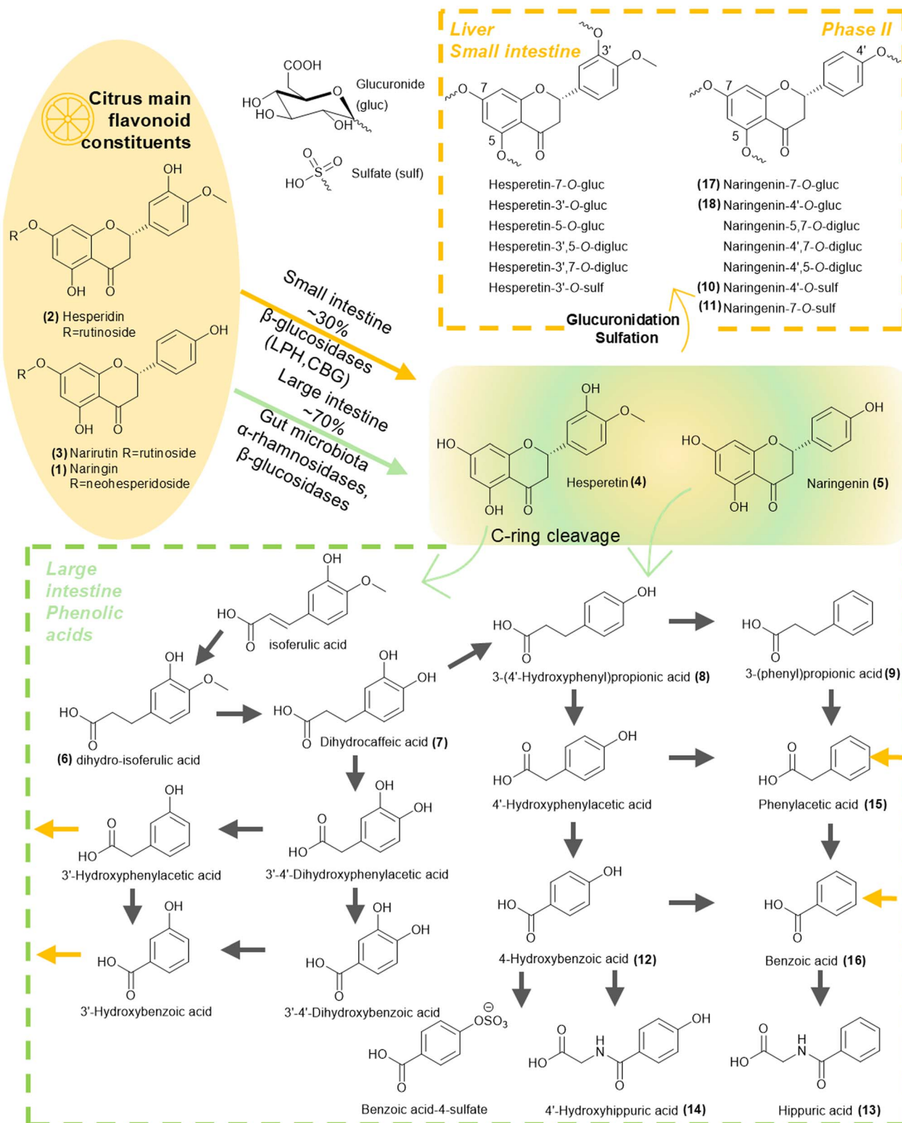
Fig. 1 Three major citrus flavonoids are hesperidin, narirutin and naringin. They are metabolized by approx. 30% in small intestine mainly through the activity of β-glucosidase and lactase phlorizin hydrolase (CBG, LPH, accordingly). The metabolization degree is higher in the large intestine (approx. 70%) due to the activity of α-rhamnosidase and β-glucosidase. In both cases, aglycone forms are liberated. Different glucuronides and sulfates are formed based on the basic scaffold structural motifs mainly in the liver and through phase II metabolism. During catabolism, phenolic acids are the main metabolites after the cleavage of C ring of the flavanones. Different derivatives of ferulic, phenylacetic and benzoic acids are produced together with hippuric acid and its derivatives. 26–28
