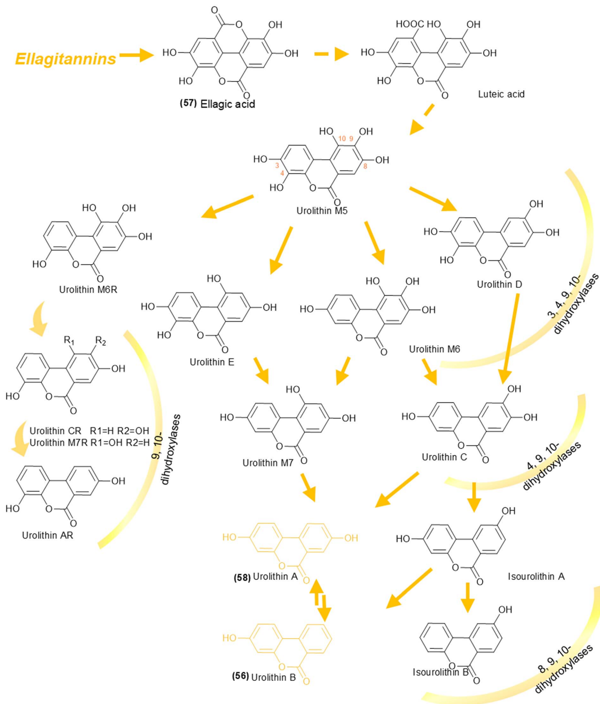
Fig. 8 Ellagitannins and ellagic acid undergo extensive metabolism by the gut microbiota, including lactone-ring cleavage, decarboxylation and dihydroxylation reactions to produce 6H-dibenzo[b,d]pyran-6-one derivatives or urolithins. 149,150
