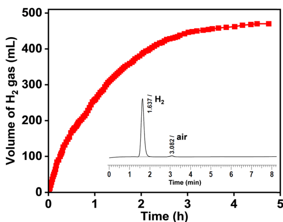
Fig. 2 Time course plot for hydrogen gas production from GLY over the \text{Ru/La}(\text{OH})_3 catalyst. Reaction conditions: \text{Ru/La}(\text{OH})_3 (100 mg, 9 wt% Ru), GLY (13.68 mmol), NaOH (27.36 mmol), water (41.04 mmol), 130 °C, and 600 rpm.
