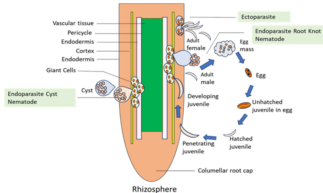
Fig. 1 Life span and mechanism of PPVs [modified from ref. 38 and 40].
