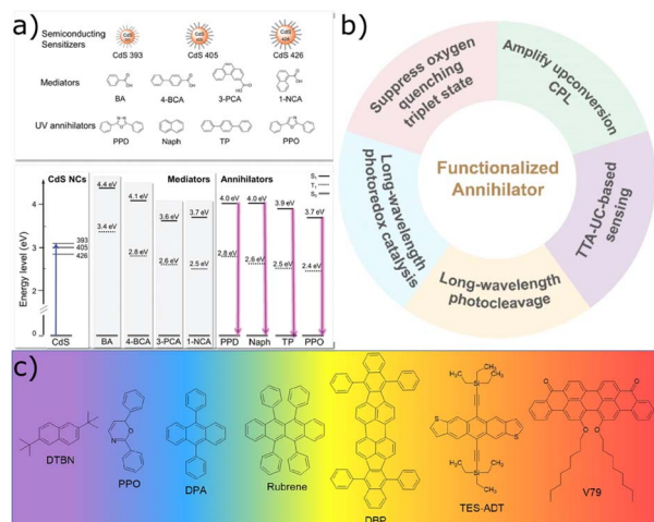
Fig. 2 (a) Illustration of semiconductor nanocrystal CdS along with the molecular structures of the four mediators and the four UV annihilators—PPD, Naph, TP, and PPO. The diagram depicting the energy levels of the CdS nanocrystals, mediators, and UV annihilators is given below. Reproduced from ref. 38 with permission from Wiley-VCH GmbH, Copyright 2021; (b) applications of functionalized annihilators. Reproduced from ref. 85 with permission from AIP Publishing, Copyright 2024; (c) chemical structures of the most used annihilator in the presence of NCs as the sensitizer. Reproduced from ref. 75 with permission from John Wiley & Sons Australia, Copyright 2024.
