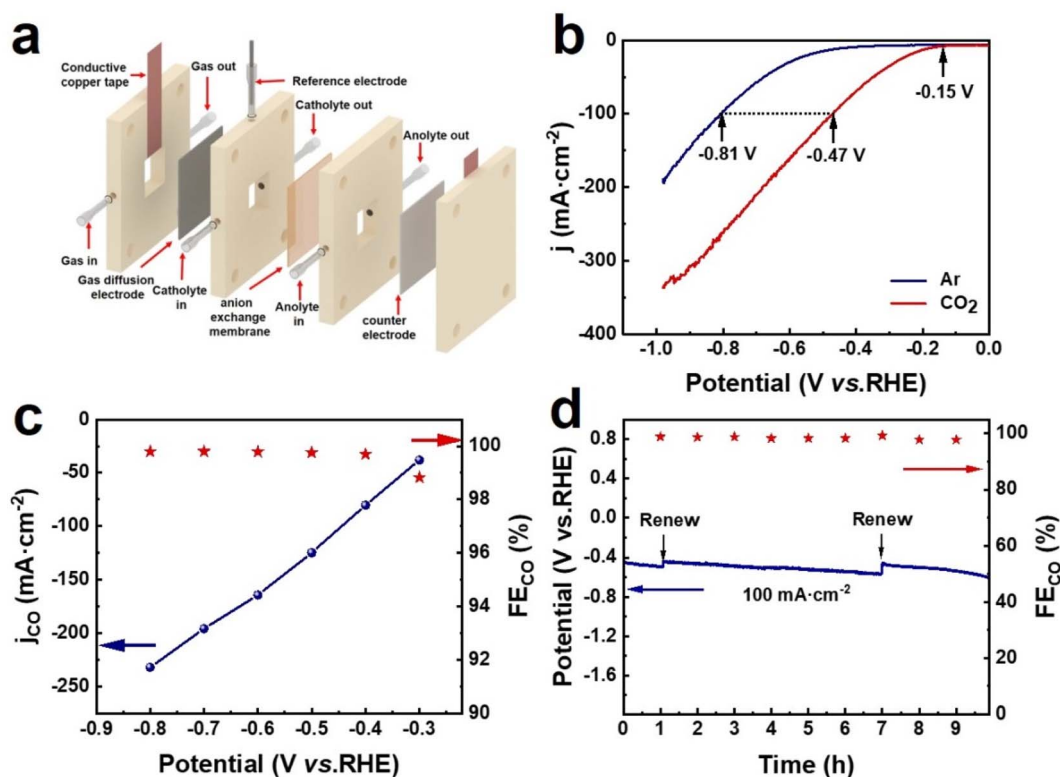
Fig. 4 (a) Schematic illustration of the flow cell electrolyzer. (b) LSV curves of the Ni-NMCF-10 catalyst under Ar or CO 2 . (c) FE CO and j CO with different applied potentials and (d) long-term stability tests of the Ni-NMCF-10 catalyst at 100 mA cm -2 in the flow cell.
