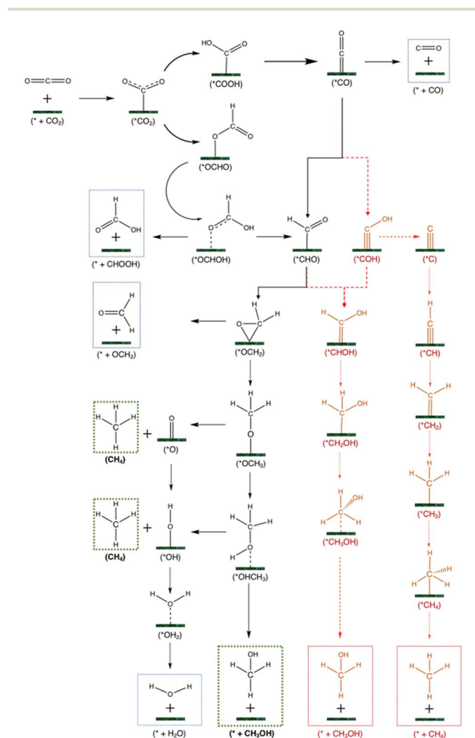
Fig. 3 Different pathways for the CO 2 RR leading to carbon monoxide, formic acid, methanol, methane, and hydrogen. Compounds with an asterisk * are adsorbed species, while compounds with no asterisk are either reactants or desorbed products. Red pathways are deemed unfavourable on most catalysts. Species in dashed boxes are final products. Products in blue boxes are intermediate, unfavourable products. Products in green boxes are the targeted products in this study: methanol and methane.
